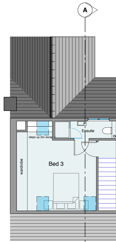
SECOND FLOOR 23 sqm
