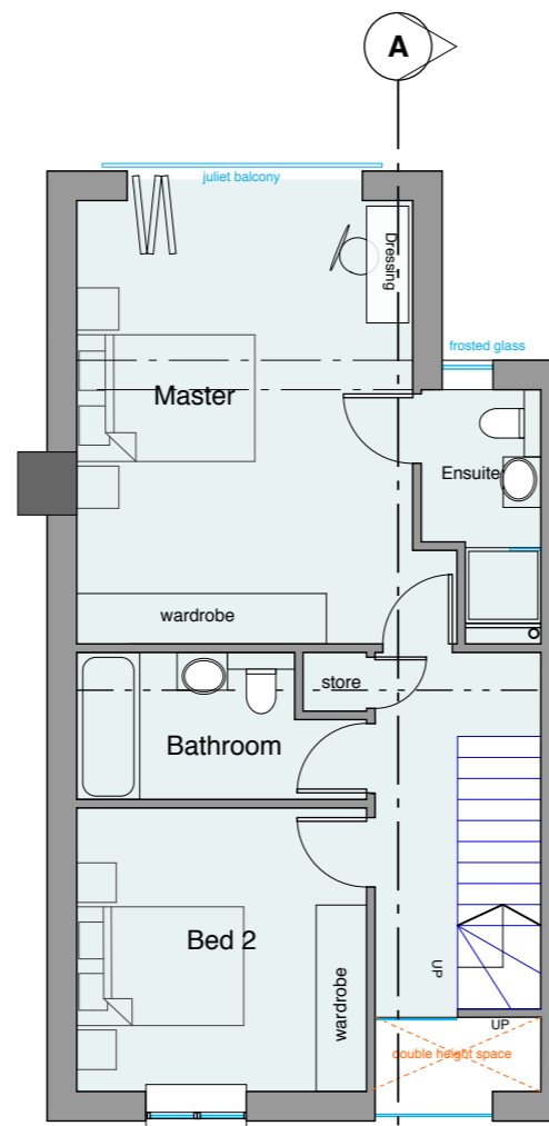
FIRST FLOOR 52.5 sqm
