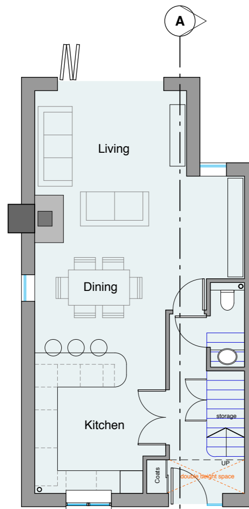
GROUND FLOOR 56 sqm
